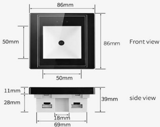
Dimensions of the ID IDENT 1500
